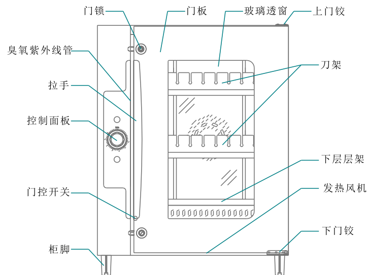
XDZ180-NDJ2
